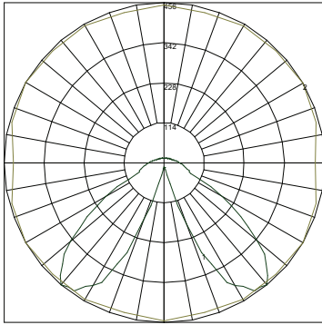
Maximum Candela = 455.603 Located At Horizontal Angle = 330, Vertical Angle = 40 # 1 - Vertical Plane Through Horizontal Angles (330 - 150) (Through Max. Cd.) # 2 - Horizontal Plane Through Vertical Angle (60) (Through Max. Cd.)
